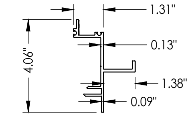
H ALUM. FRAME MEMBER
