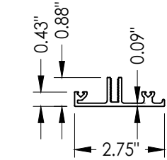
D HORIZONTAL MEMBER
