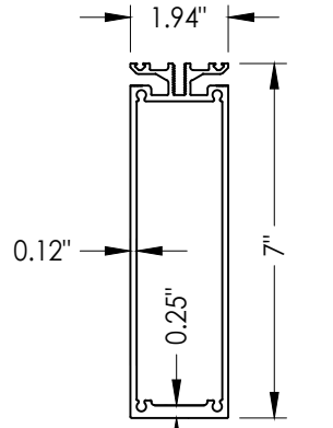
1 SERIES 700 RAFTER Optional
