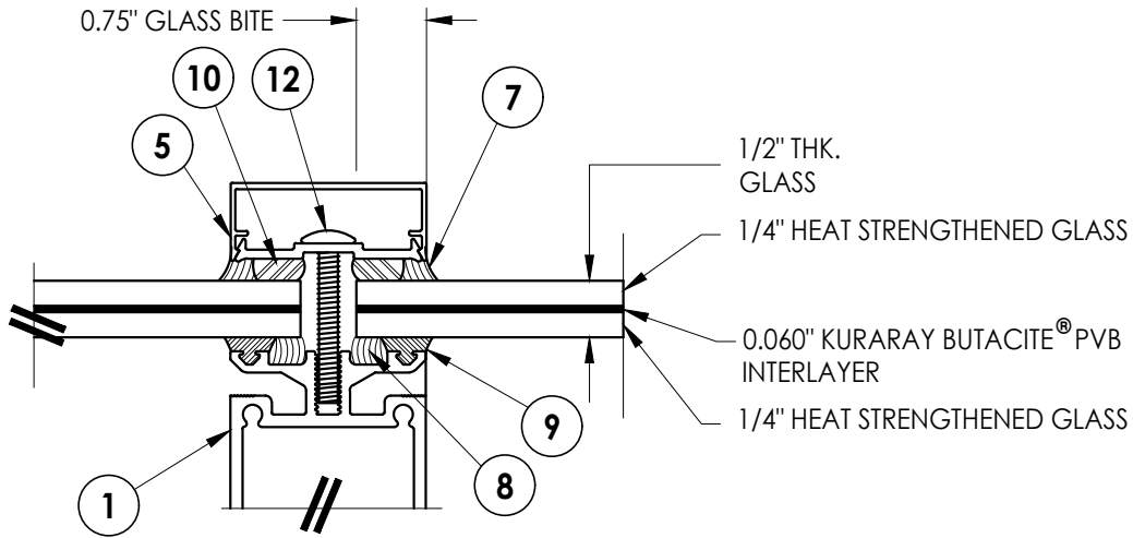
G4 GLAZING DETAIL
