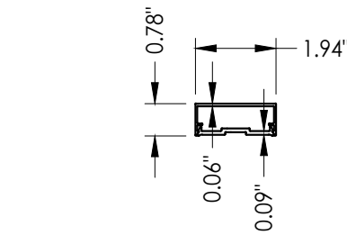
B COMPRESSION PLATE & COVER
