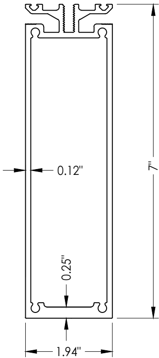
1 SERIES 700 RAFTER Optional
