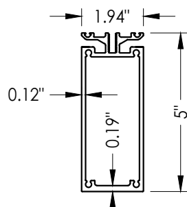
1 SERIES 500 RAFTER Optional
