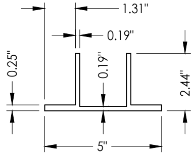
G BRAC-1 SADDLE CLIP 2" wide
